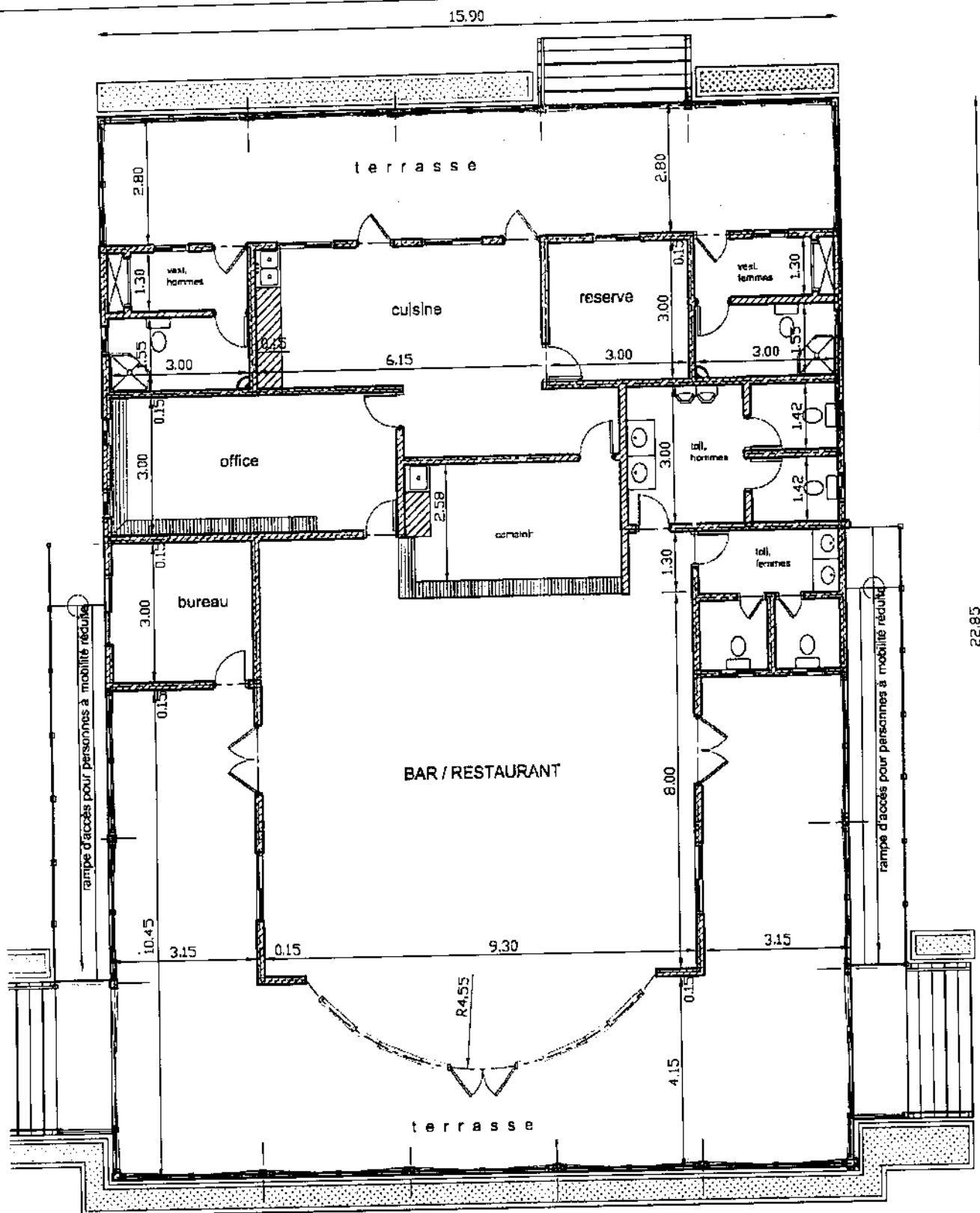
PLAN DU BAR/RESTAURANT
